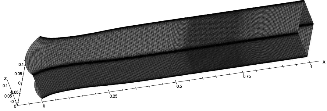
Fig. 3 Typical computational mesh used for steady and unsteady calculations (3,300,000 cells).
