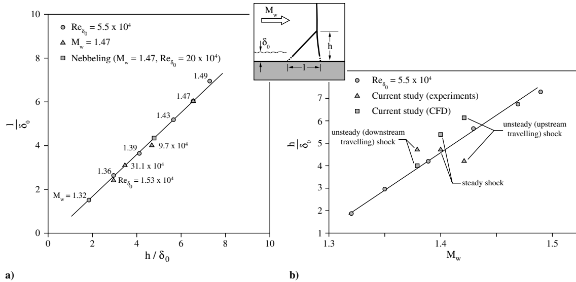
Fig. 13 Variation of steady transonic SBLI geometry with Mach number: a) bifurcation topography and b) effect of Mach number on bifurcation (triple-point) height. The parameters l , h , \delta_0 , and M_w used in the plots are defined in the (inset) schematic diagram. Figures are adapted from Doerffer [17].
